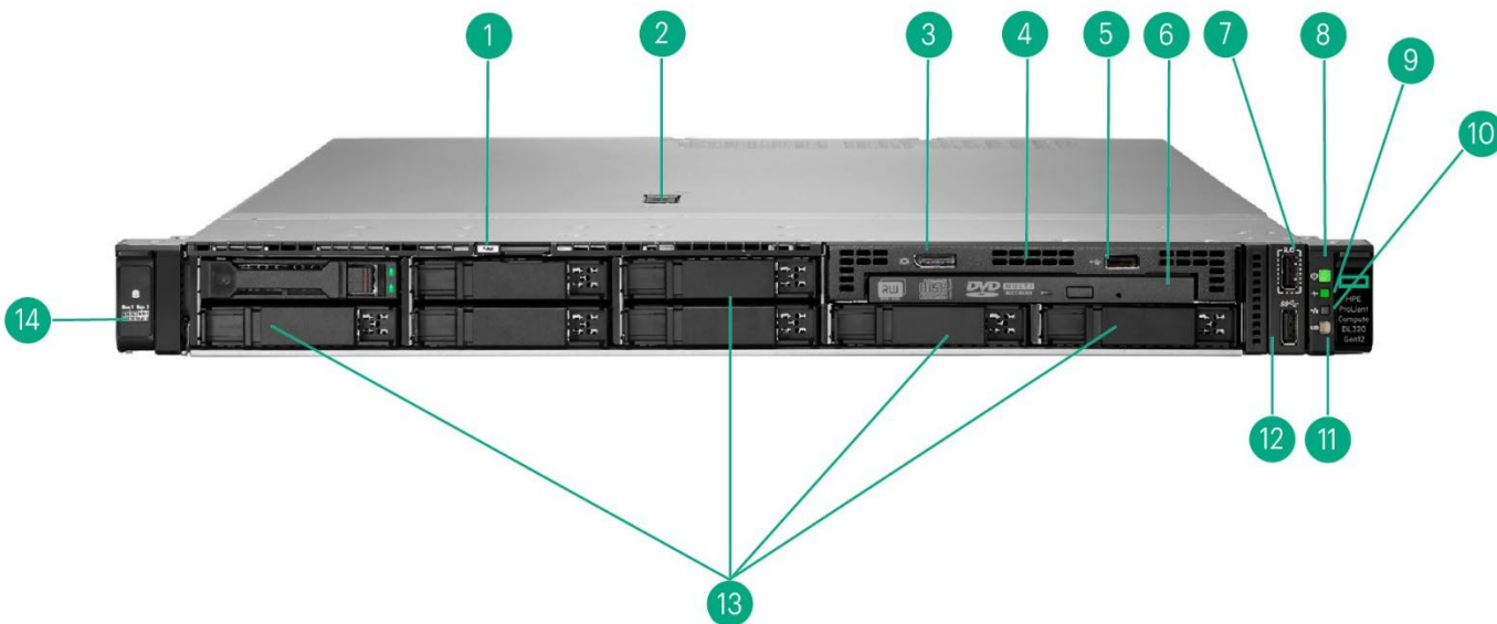
SFF Front View with optional Universal Media Bay, optical Drive, DisplayPort, USB 2.0
